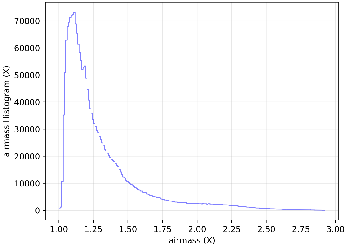
weather_cloudso1v3.4_10yrs All sky all bands: airmass Histogram
