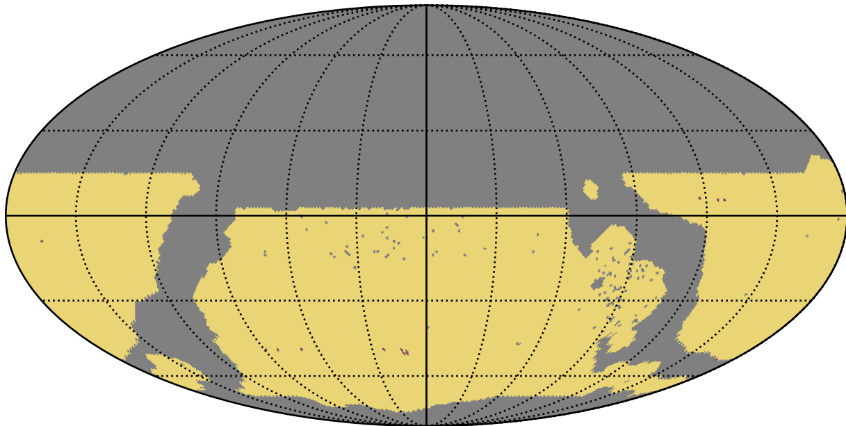
weather_cloudso1v3.4_10yrs WFD: RapidRevisits
