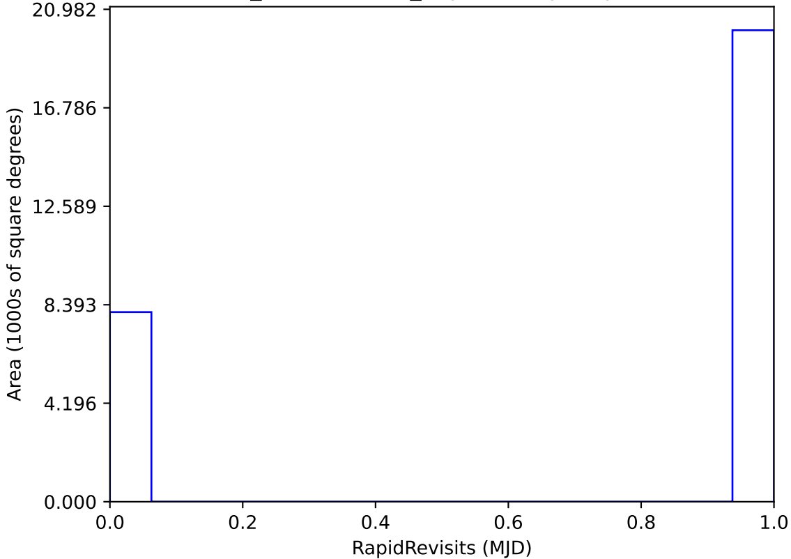
weather_cloudso1v3.4_10yrs All sky: RapidRevisits
