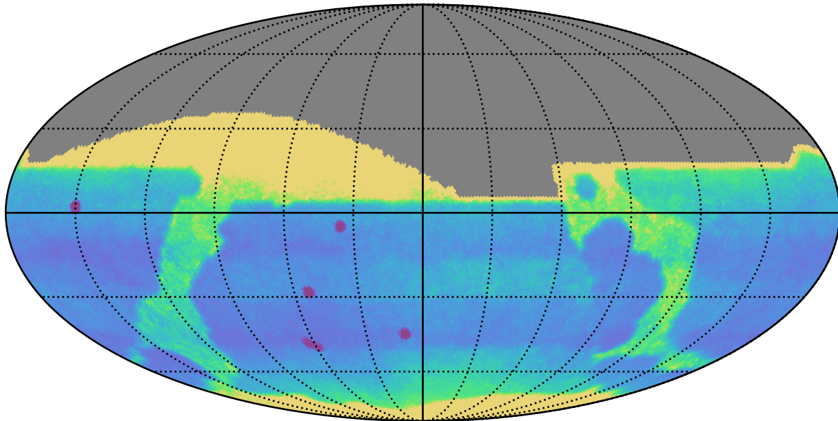
weather_cloudso1v3.4_10yrs All sky: Proper Motion Uncert @ 24.0
