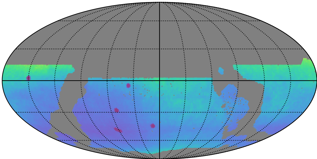
weather_cloudso1v3.4_10yrs WFD: Parallax Uncert @ 22.4
