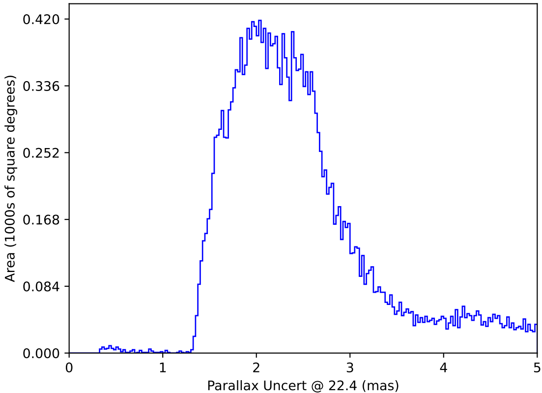
weather_cloudso1v3.4_10yrs All sky: Parallax Uncert @ 22.4
