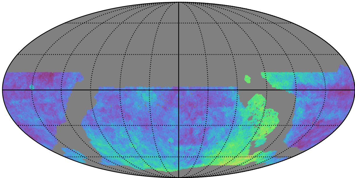
weather_cloudso1v3.4_10yrs WFD: Parallax Coverage @ 24.0
