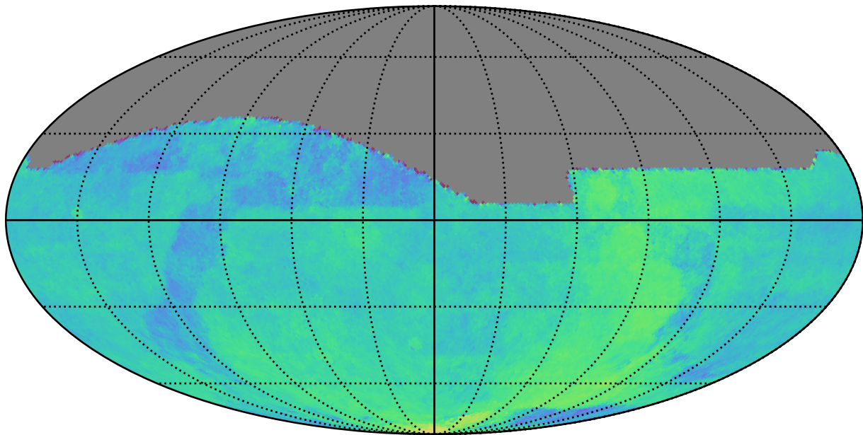
weather_cloudso1v3.4_10yrs All sky: Parallax Coverage @ 24.0
