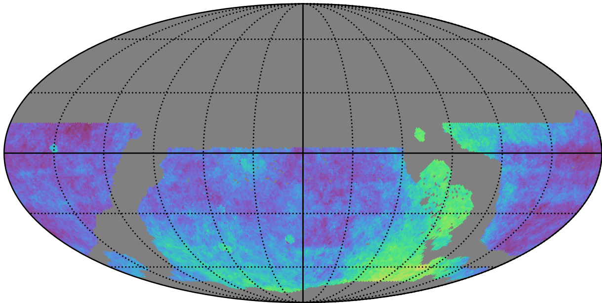
weather_cloudso1v3.4_10yrs WFD: Parallax Coverage @ 22.4
