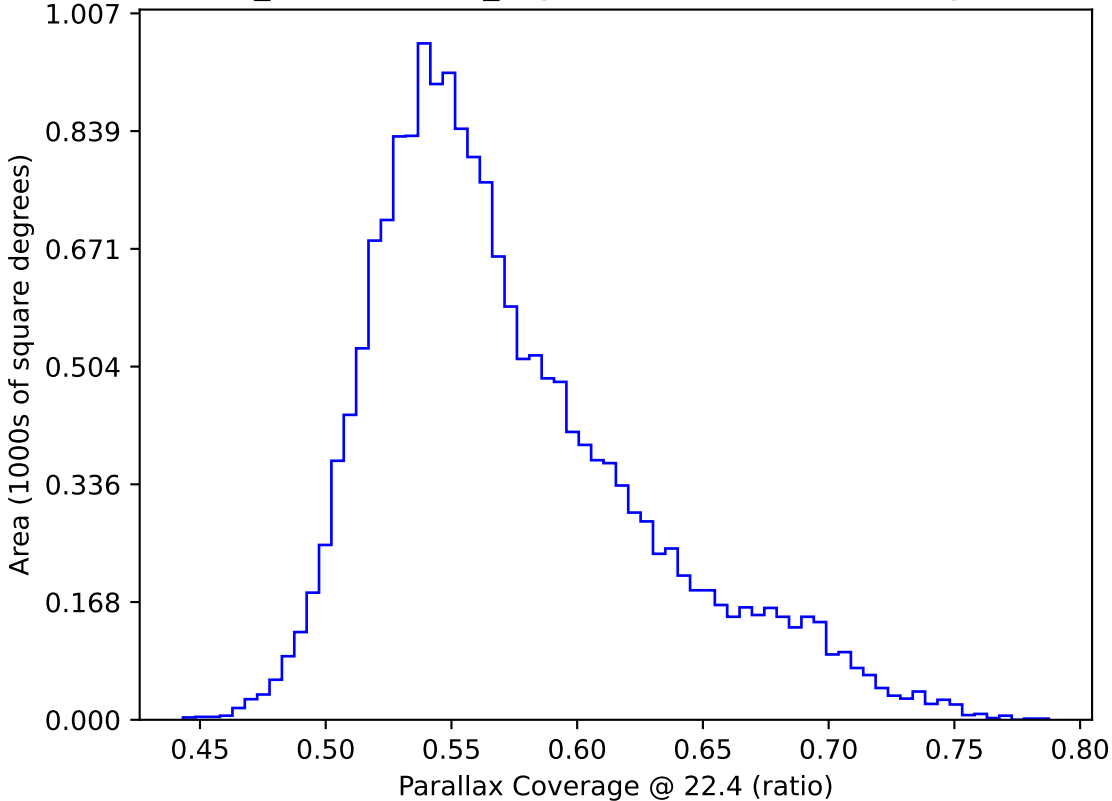
weather_cloudso1v3.4_10yrs WFD: Parallax Coverage @ 22.4
