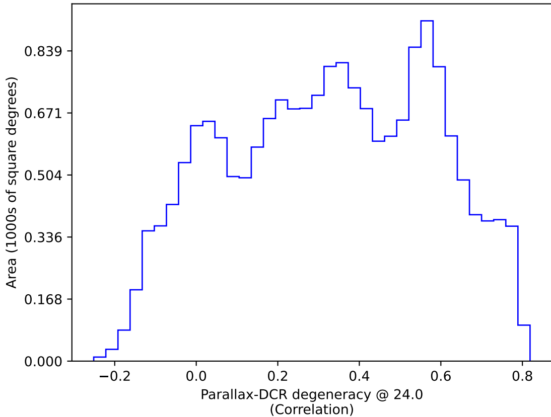
weather_cloudso1v3.4_10yrs WFD: Parallax-DCR degeneracy @ 24.0
