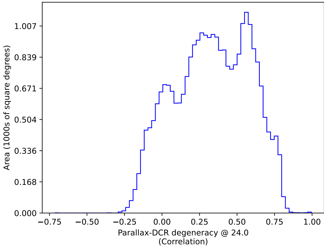
weather_cloudso1v3.4_10yrs All sky: Parallax-DCR degeneracy @ 24.0
