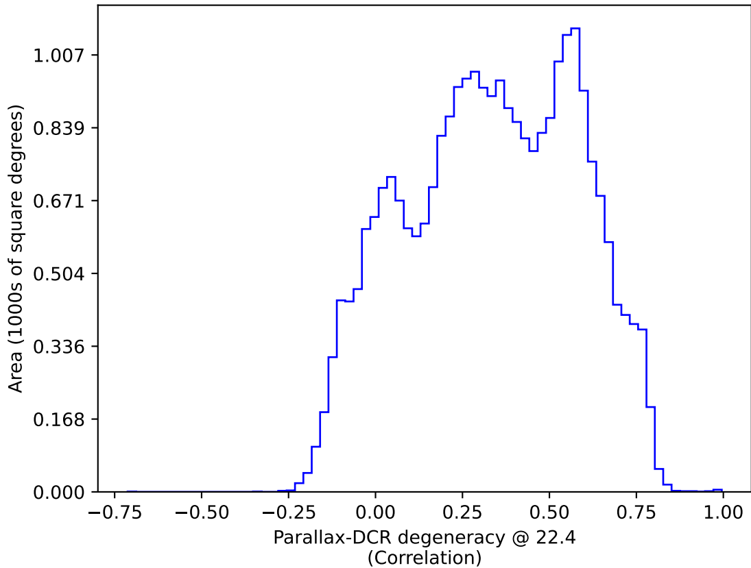
weather_cloudso1v3.4_10yrs All sky: Parallax-DCR degeneracy @ 22.4
