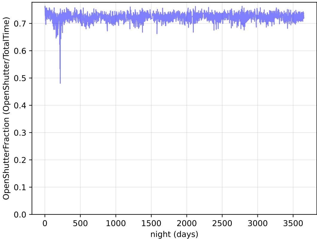
weather_cloudso1v3.4_10yrs Per night: OpenShutterFraction
