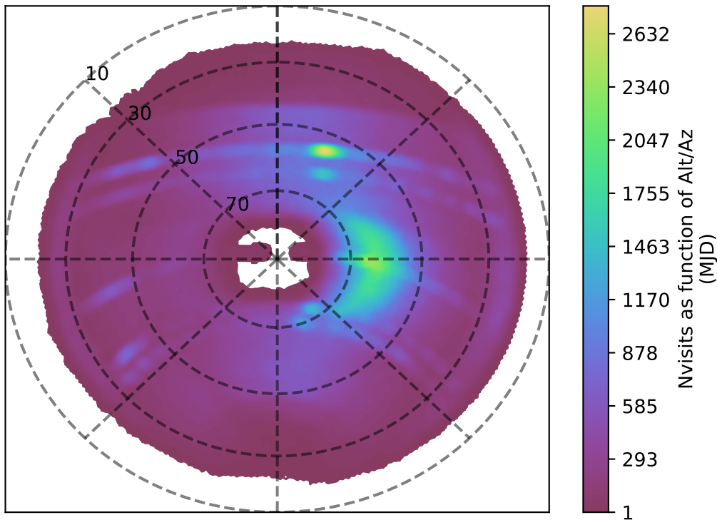
weather_cloudso1v3.4_10yrs z band: Nvisits as function of Alt/Az
