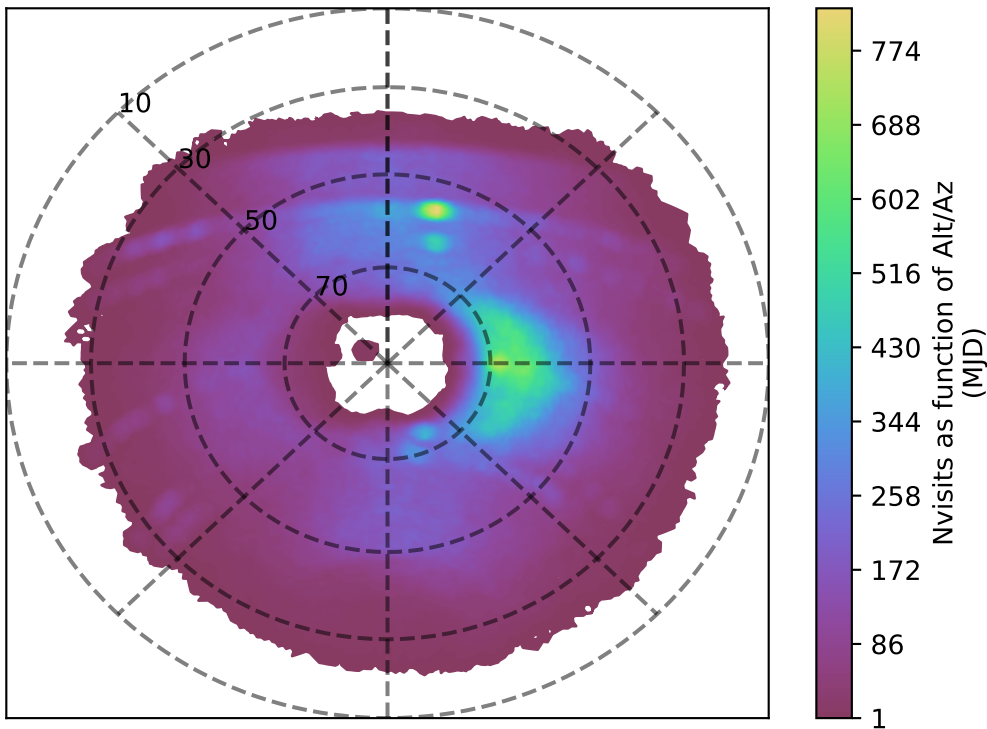
weather_cloudso1v3.4_10yrs u band: Nvisits as function of Alt/Az
