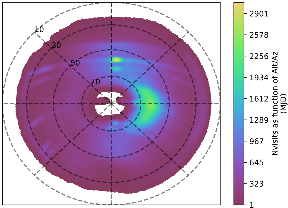
weather_cloudso1v3.4_10yrs i band: Nvisits as function of Alt/Az
