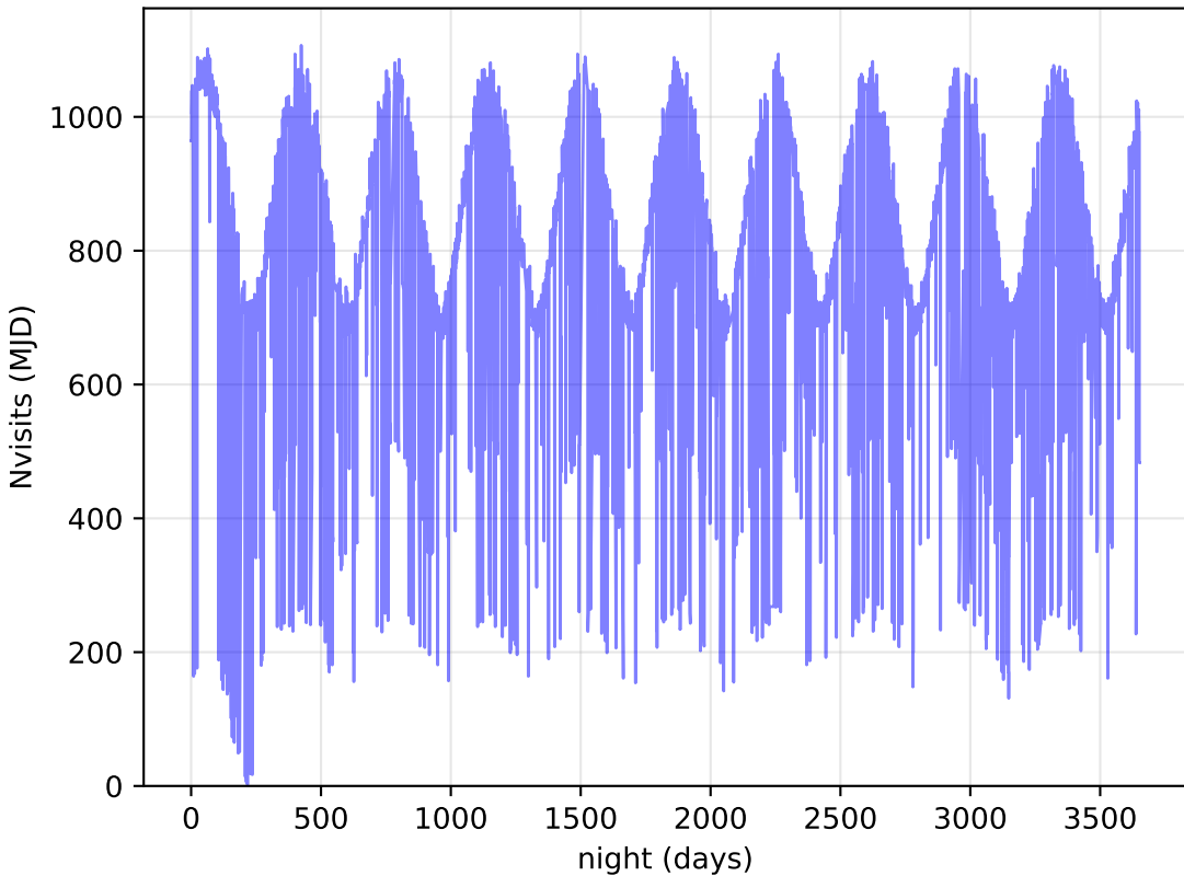
weather_cloudso1v3.4_10yrs All visits: Nvisits
