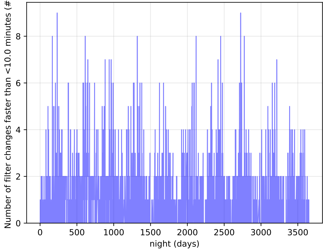
weather_cloudso1v3.4_10yrs Per Night: Number of filter changes faster than <10.0 minutes
