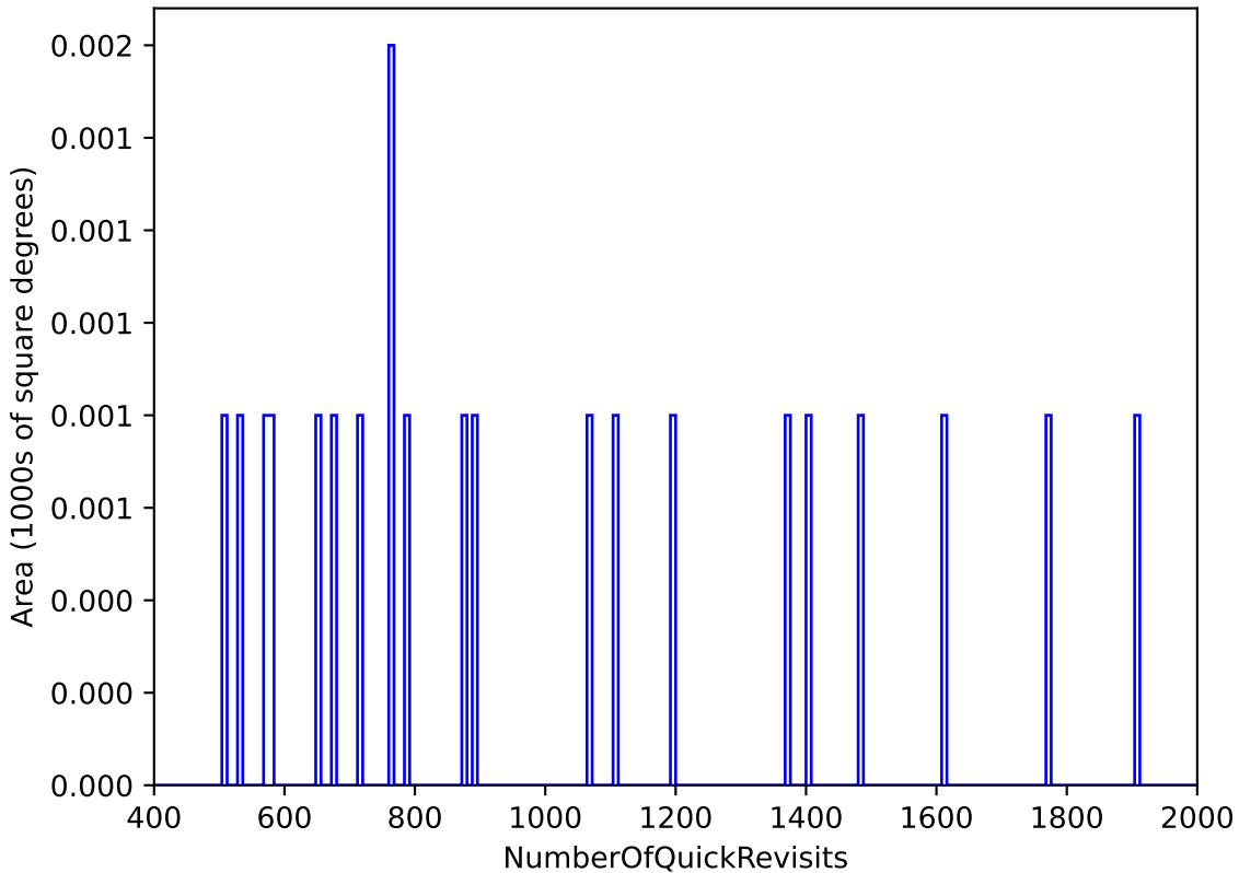
weather_cloudso1v3.4_10yrs WFD: NumberOfQuickRevisits
