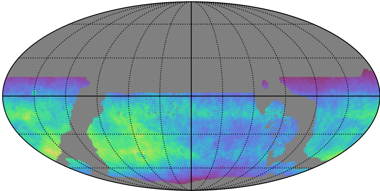
weather_cloudso1v3.4_10yrs WFD z band: Normalized Teff
