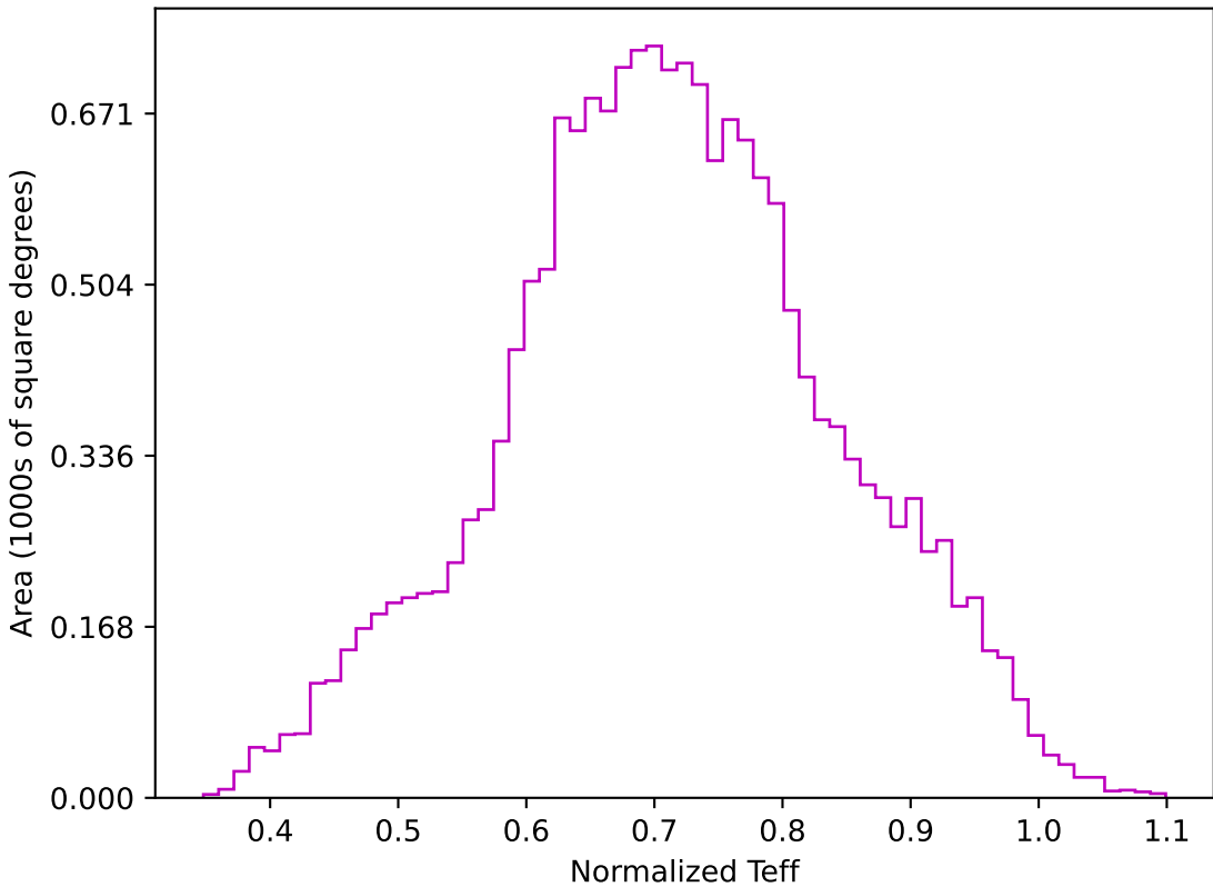
weather_cloudso1v3.4_10yrs WFD z band: Normalized Teff
