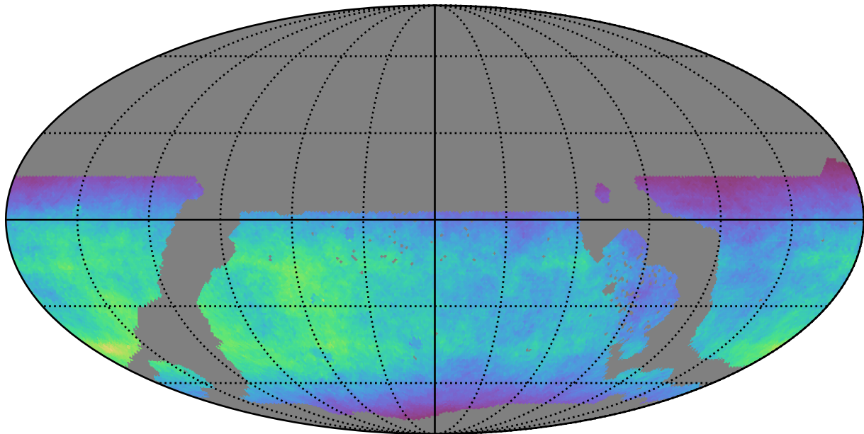
weather_cloudso1v3.4_10yrs WFD y band: Normalized Teff
