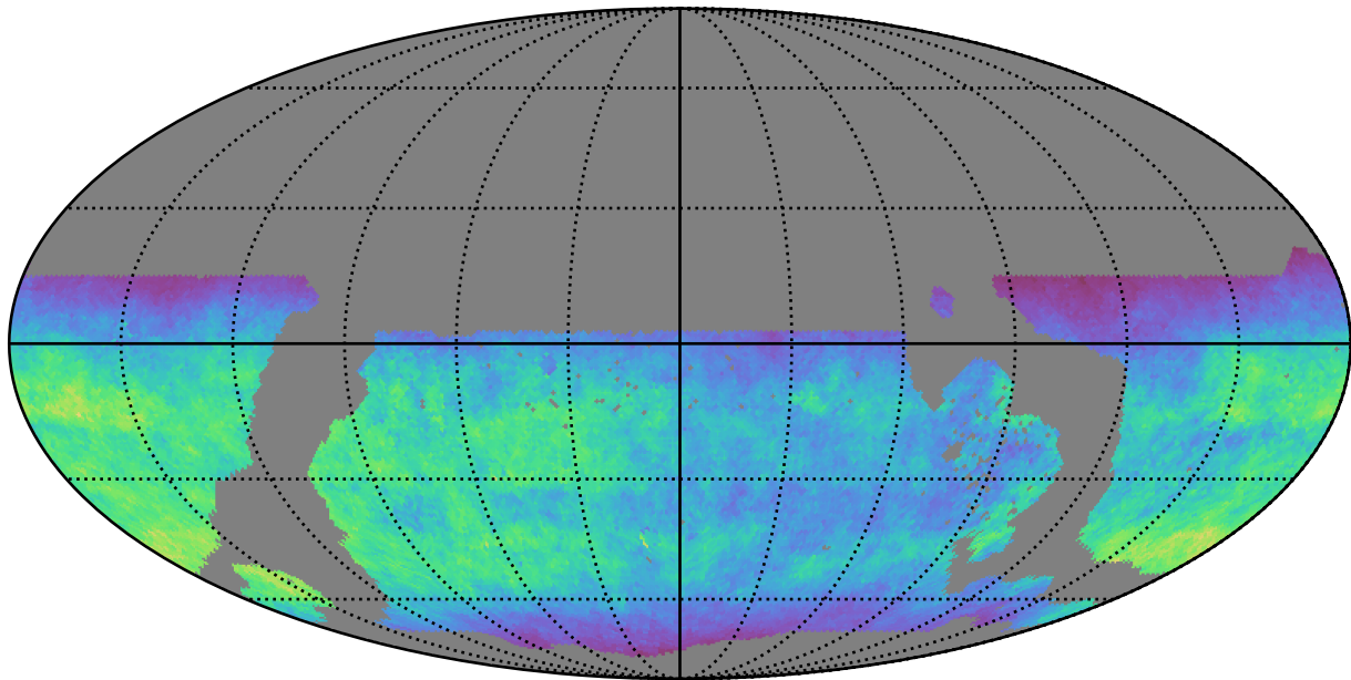
weather_cloudso1v3.4_10yrs WFD u band: Normalized Teff
