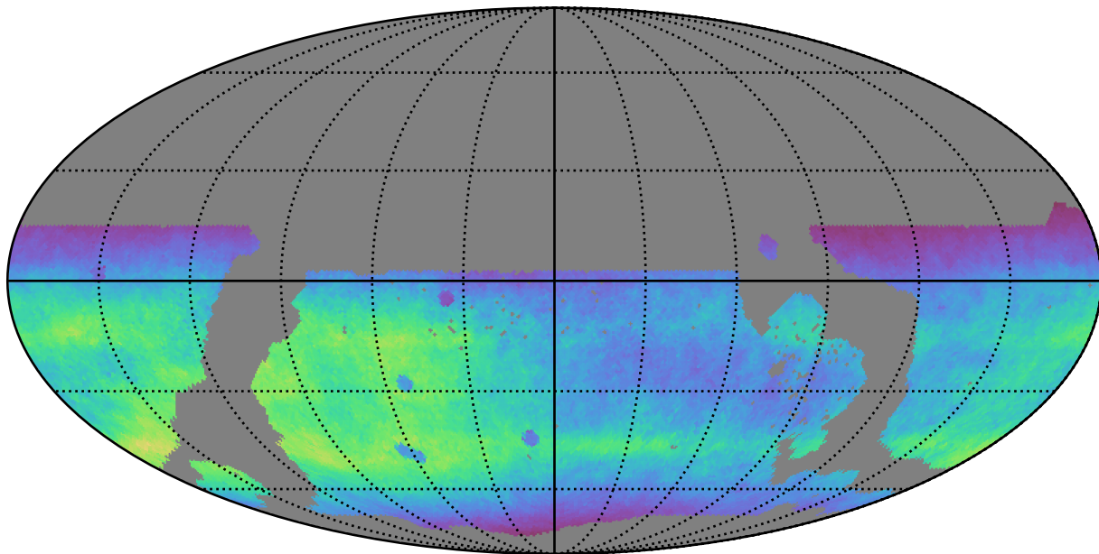
weather_cloudso1v3.4_10yrs WFD r band: Normalized Teff
