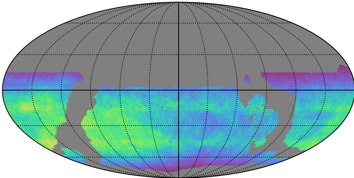
weather_cloudso1v3.4_10yrs WFD i band: Normalized Teff
