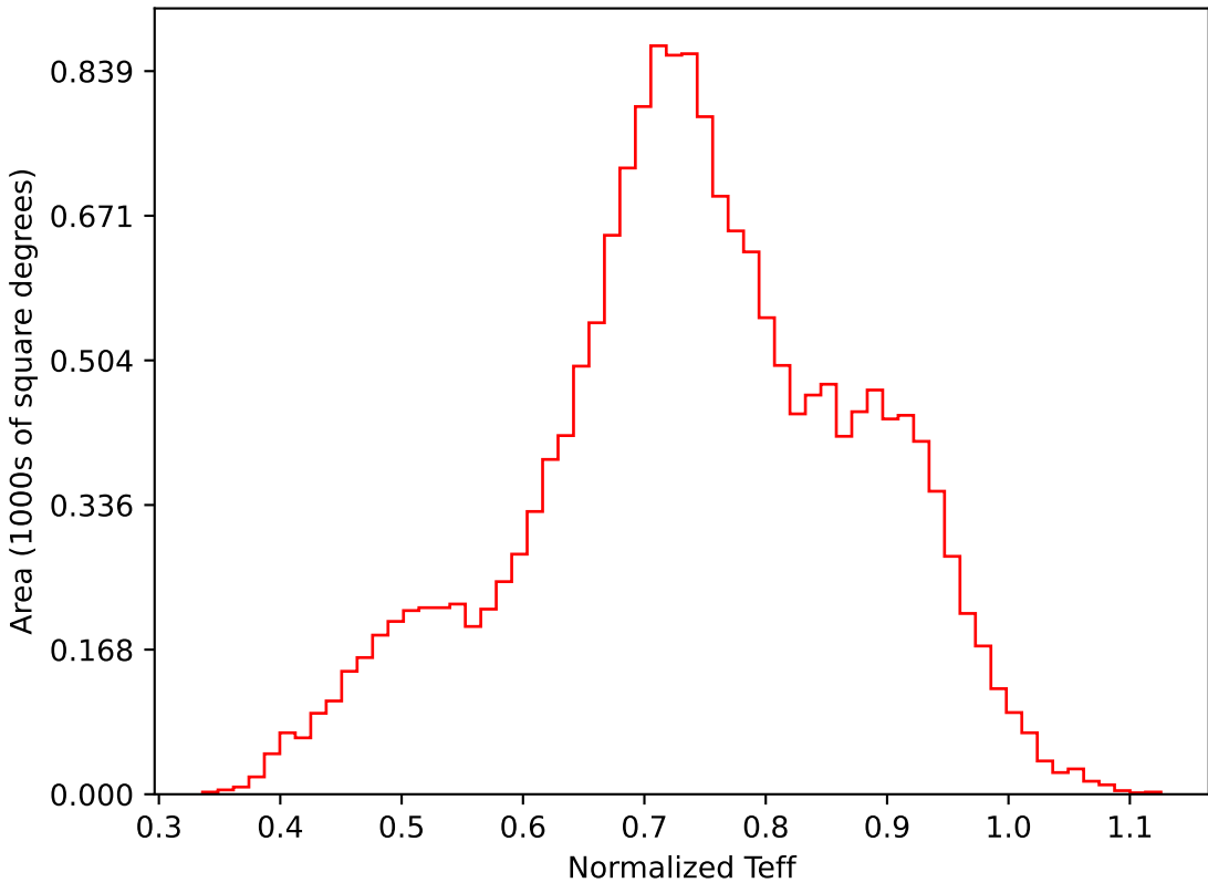
weather_cloudso1v3.4_10yrs WFD i band: Normalized Teff
