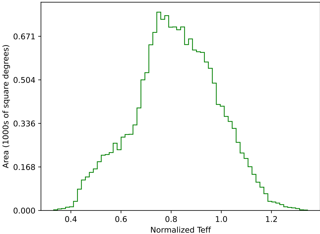
weather_cloudso1v3.4_10yrs WFD g band: Normalized Teff
