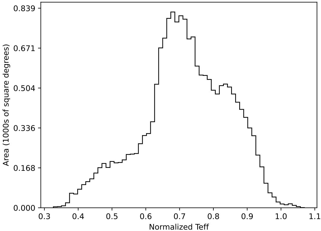
weather_cloudso1v3.4_10yrs WFD all bands: Normalized Teff
