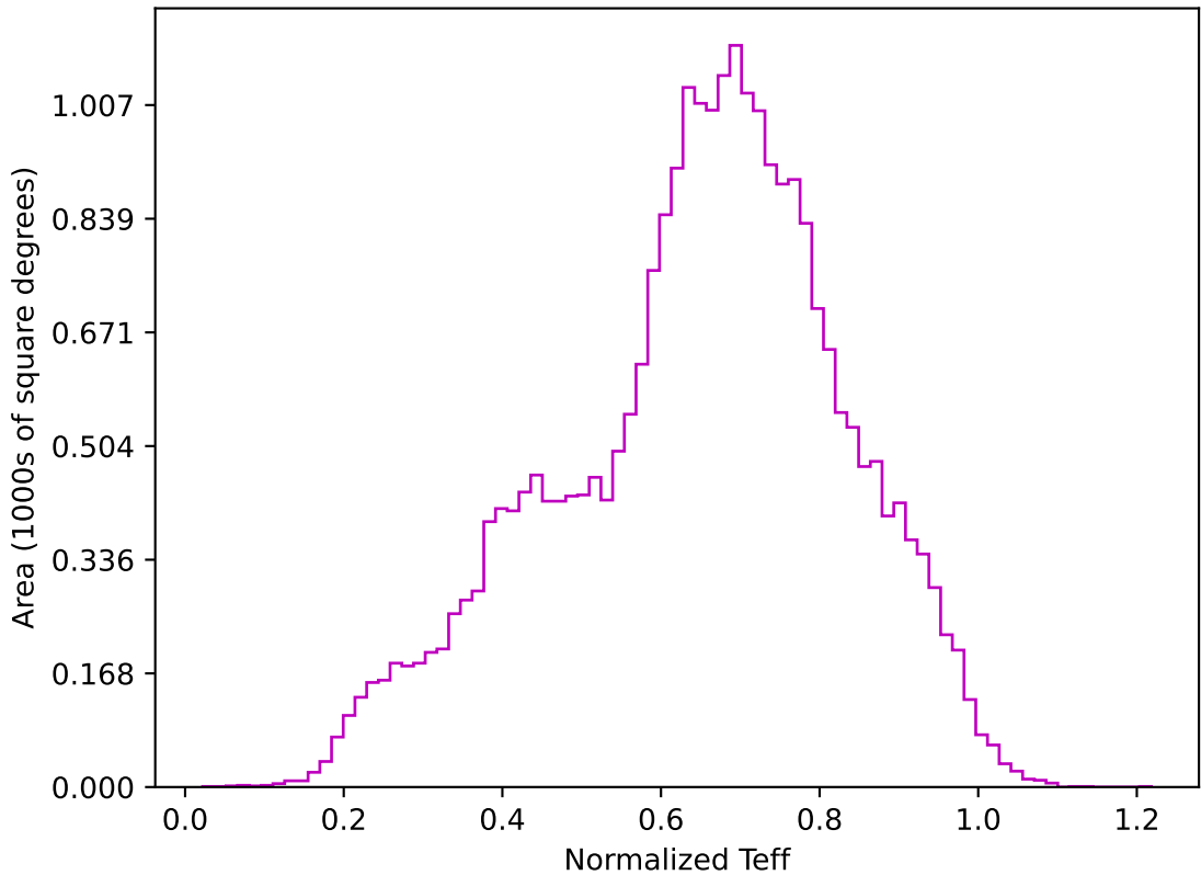
weather_cloudso1v3.4_10yrs All sky z band: Normalized Teff
