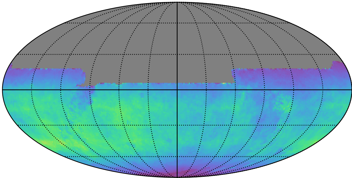
weather_cloudso1v3.4_10yrs All sky y band: Normalized Teff
