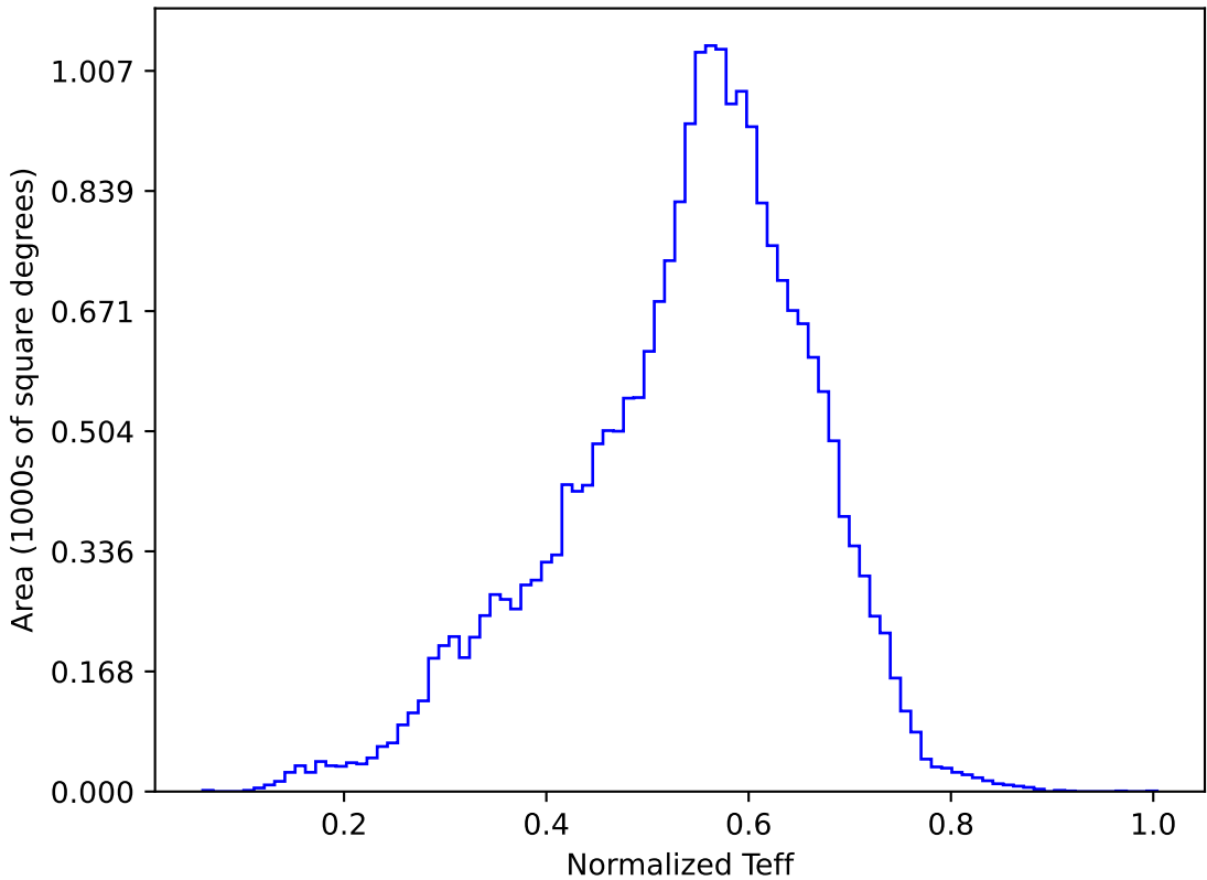
weather_cloudso1v3.4_10yrs All sky y band: Normalized Teff
