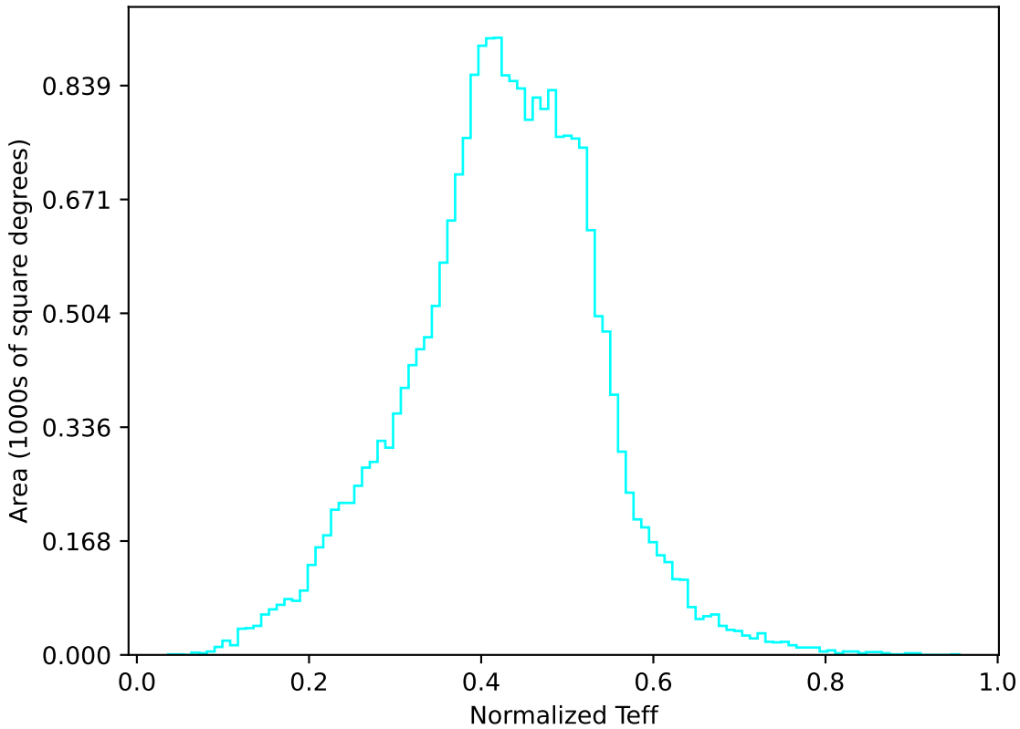
weather_cloudso1v3.4_10yrs All sky u band: Normalized Teff
