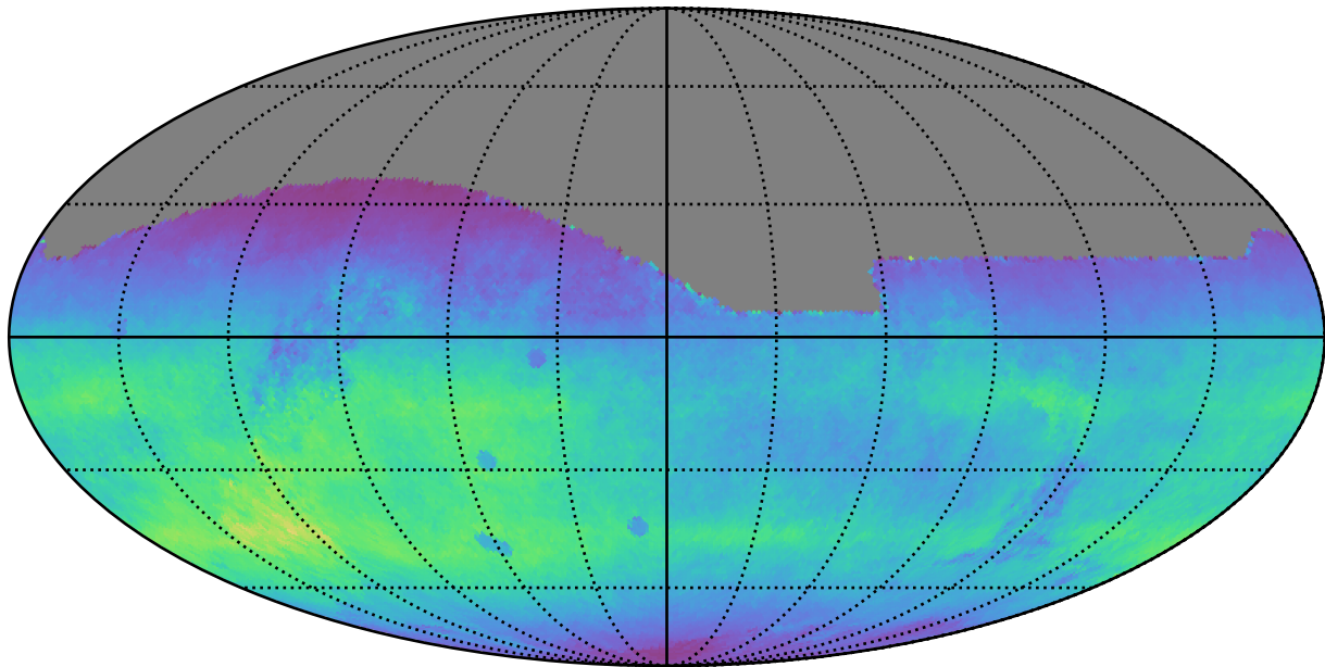
weather_cloudso1v3.4_10yrs All sky r band: Normalized Teff
