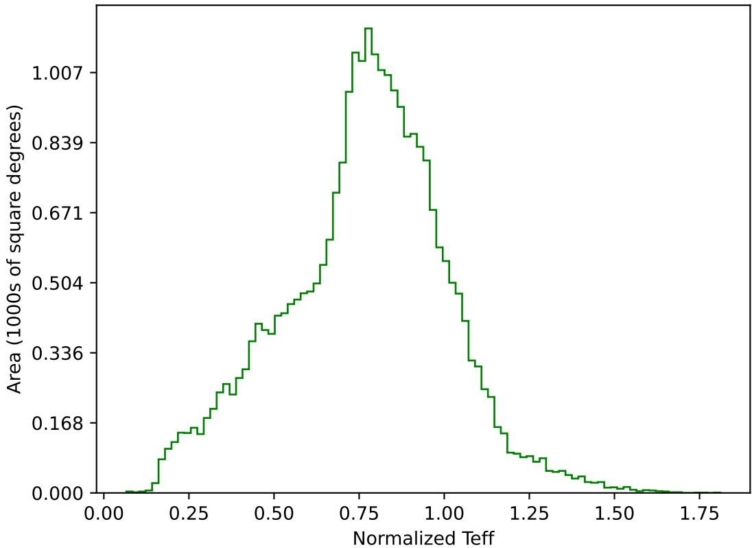
weather_cloudso1v3.4_10yrs All sky g band: Normalized Teff
