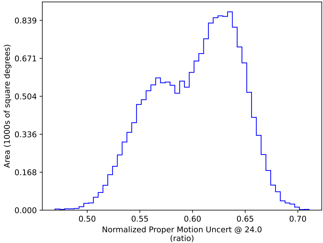
weather_cloudso1v3.4_10yrs WFD: Normalized Proper Motion Uncert @ 24.0
