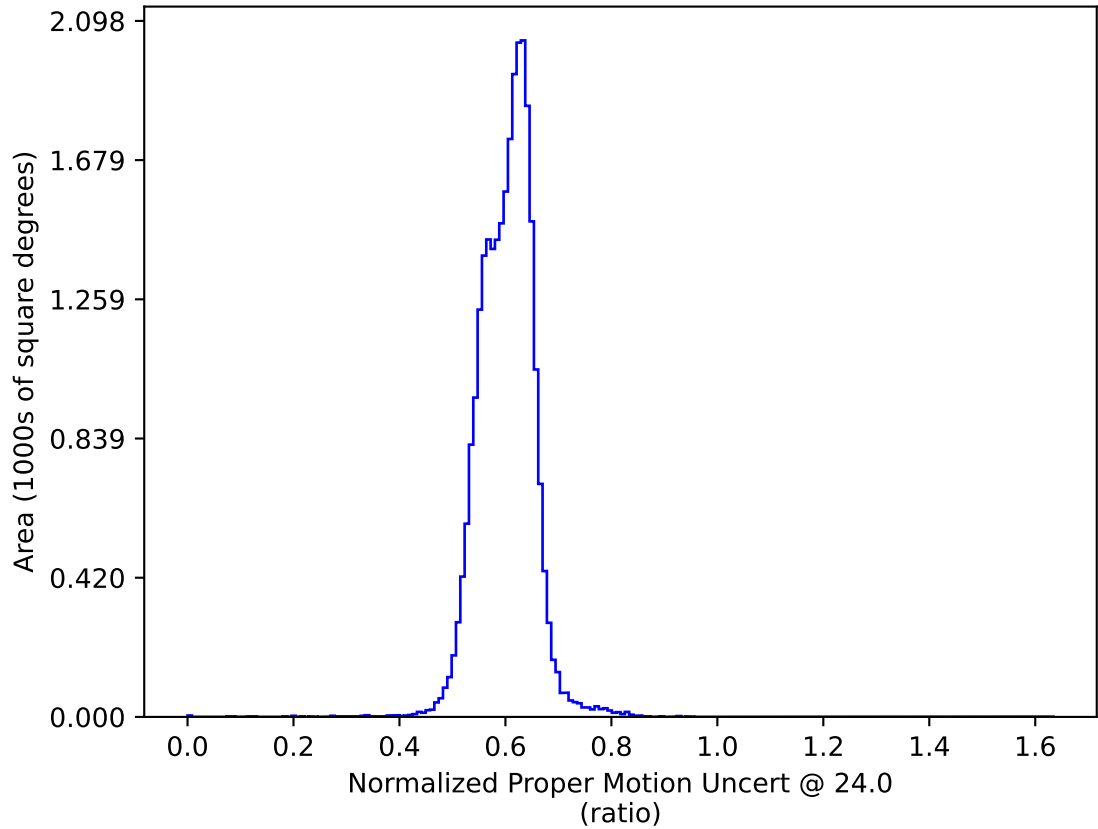
weather_cloudso1v3.4_10yrs All sky: Normalized Proper Motion Uncert @ 24.0
