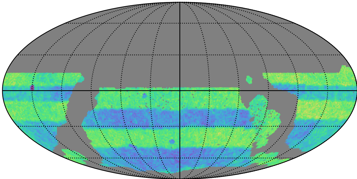
weather_cloudso1v3.4_10yrs WFD: Normalized Proper Motion Uncert @ 20.5
