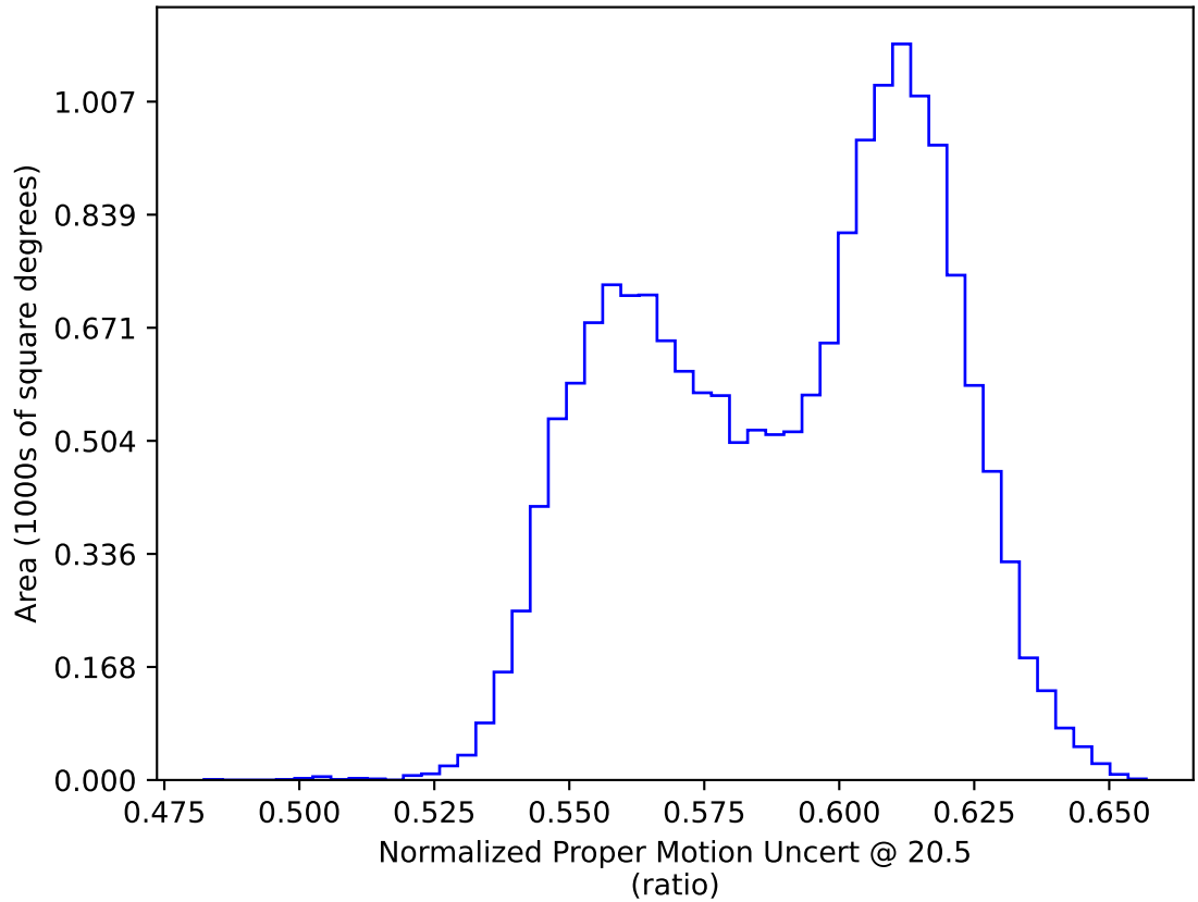
weather_cloudso1v3.4_10yrs WFD: Normalized Proper Motion Uncert @ 20.5
