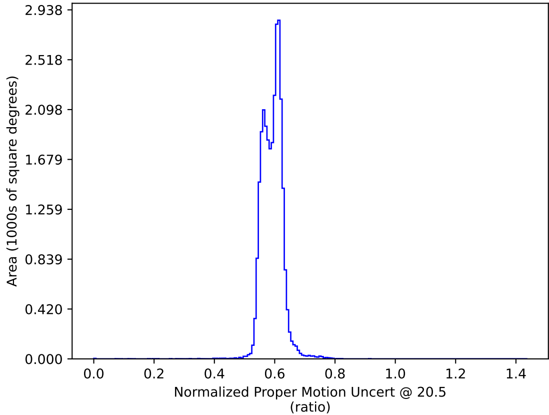
weather_cloudso1v3.4_10yrs All sky: Normalized Proper Motion Uncert @ 20.5
