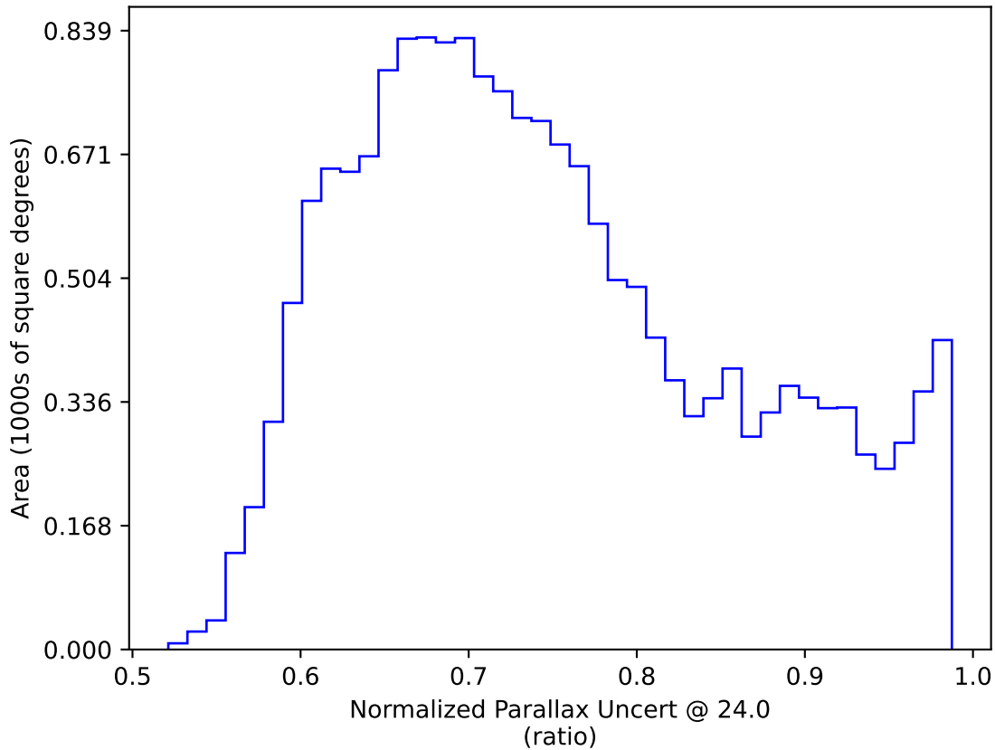
weather_cloudso1v3.4_10yrs WFD: Normalized Parallax Uncert @ 24.0
