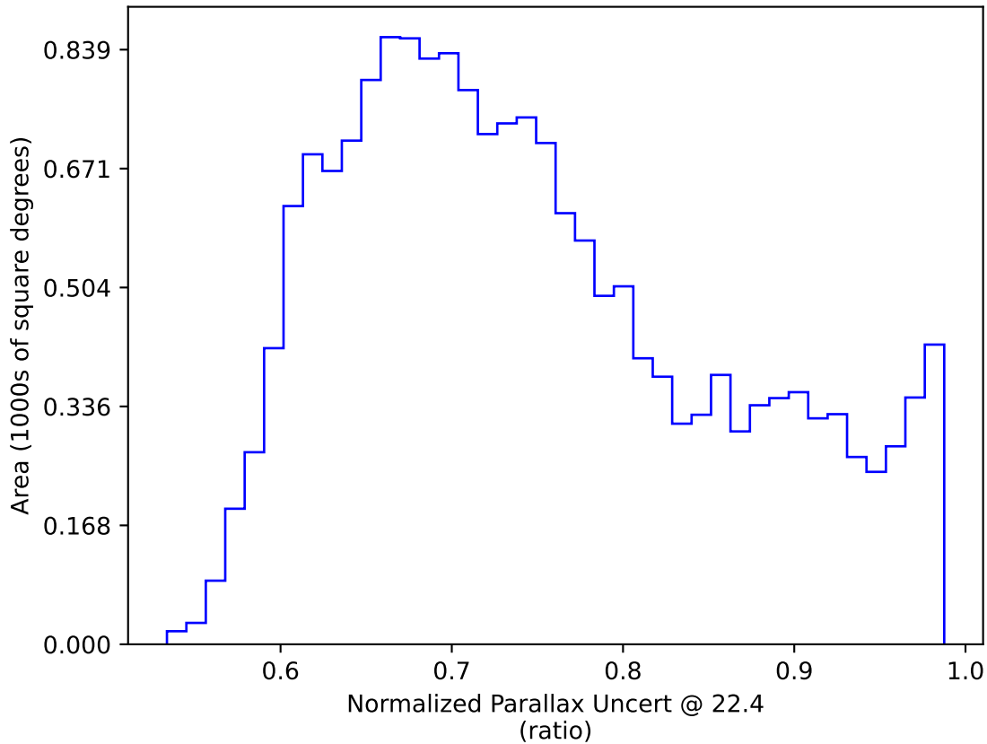
weather_cloudso1v3.4_10yrs WFD: Normalized Parallax Uncert @ 22.4
