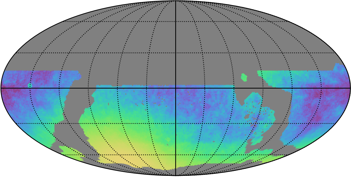
weather_cloudso1v3.4_10yrs WFD y band only: Normalized Parallax Uncert @ 21.3
