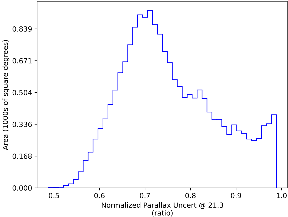
weather_cloudso1v3.4_10yrs WFD y band only: Normalized Parallax Uncert @ 21.3
