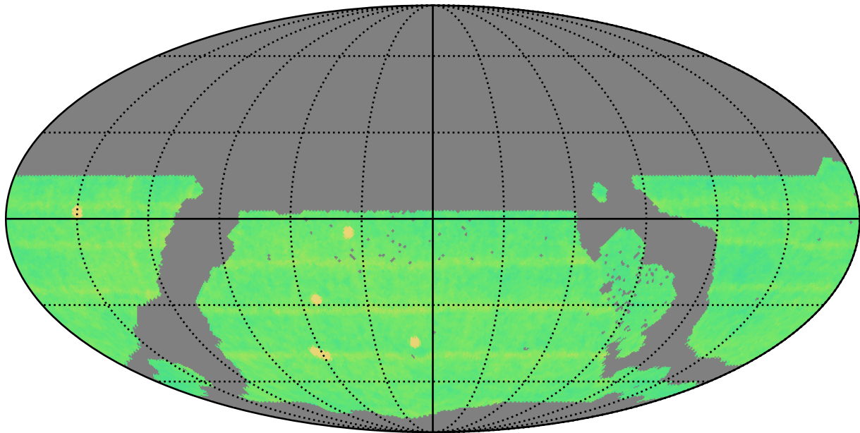
weather_cloudso1v3.4_10yrs WFD all bands: N Unique Nights
