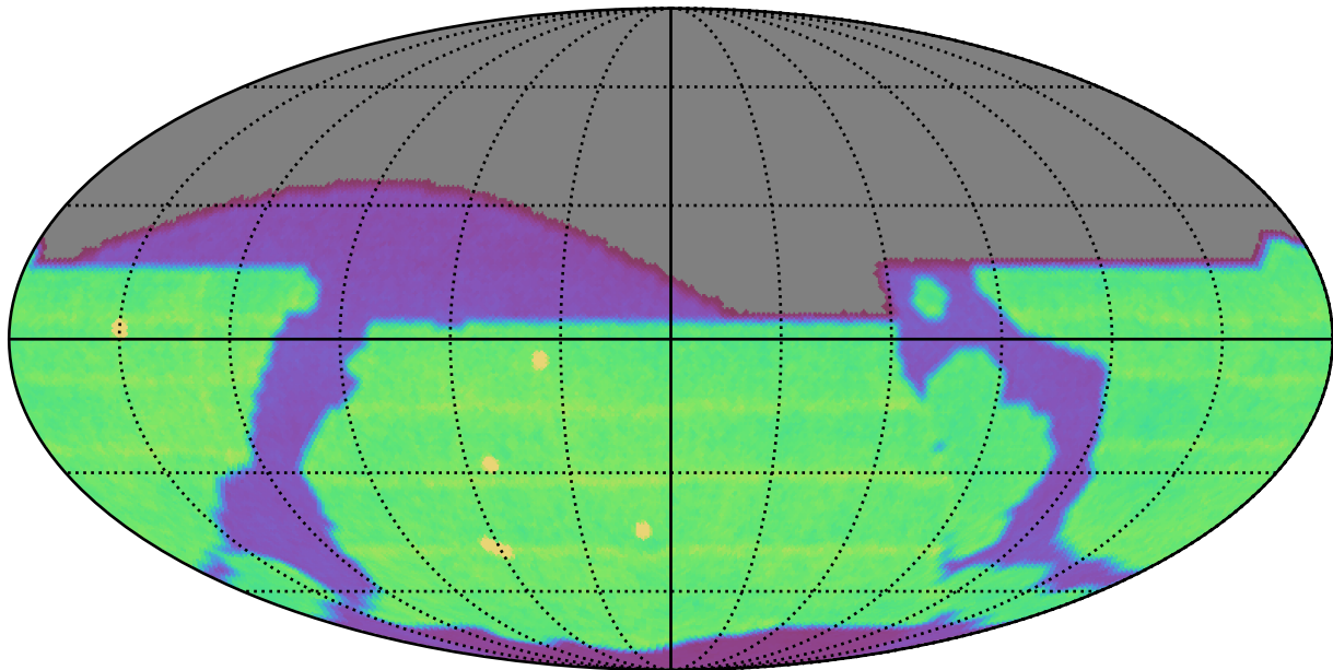
weather_cloudso1v3.4_10yrs All sky all bands: N Unique Nights
