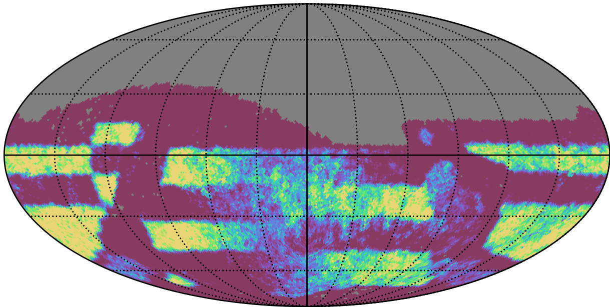
weather_cloudso1v3.4_10yrs Yr 3-4 z band: NVisits
