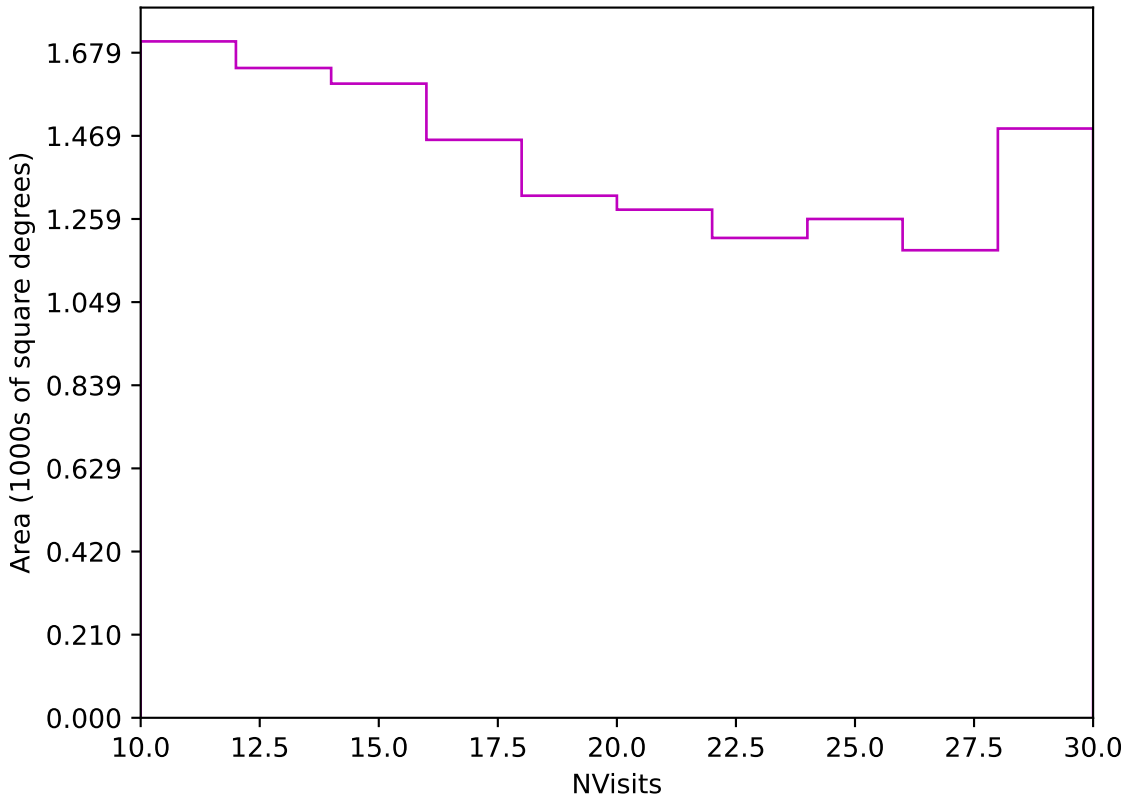
weather_cloudso1v3.4_10yrs Yr 3-4 z band: NVisits
