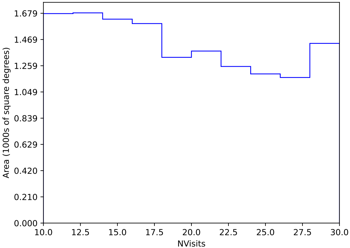
weather_cloudso1v3.4_10yrs Yr 3-4 y band: NVisits
