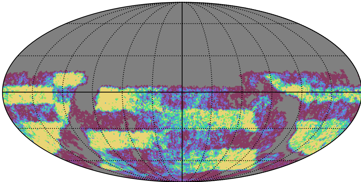
weather_cloudso1v3.4_10yrs Yr 3-4 u band: NVisits
